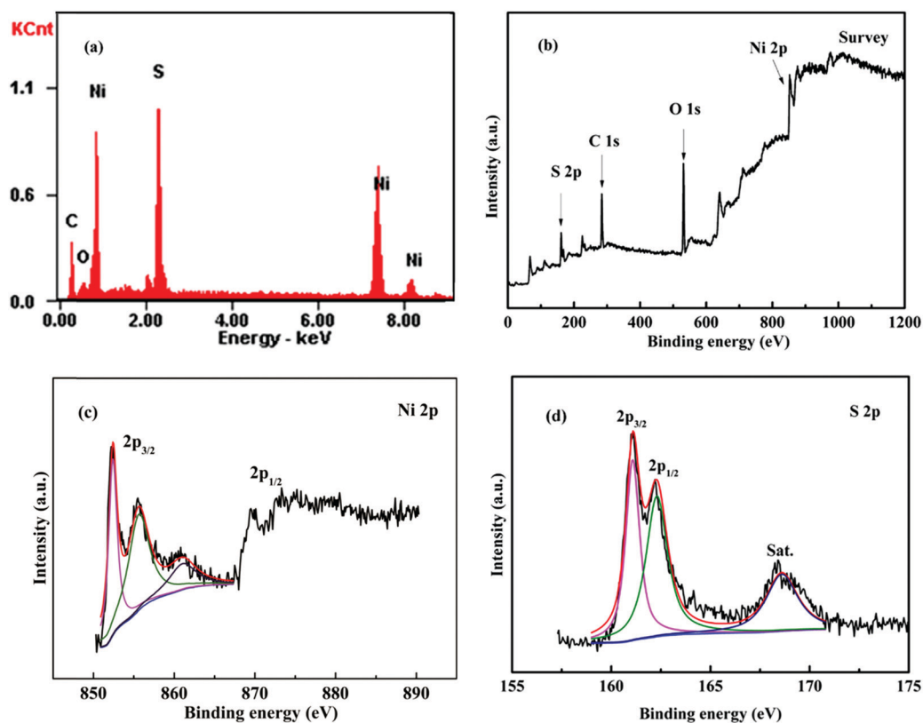
Fig. 4 (a) EDS pattern of Ni–S-10 h; XPS spectra of Ni–S-10 h: (b) survey spectrum, (c) Ni 2p spectrum, and (d) S 2p spectrum.
