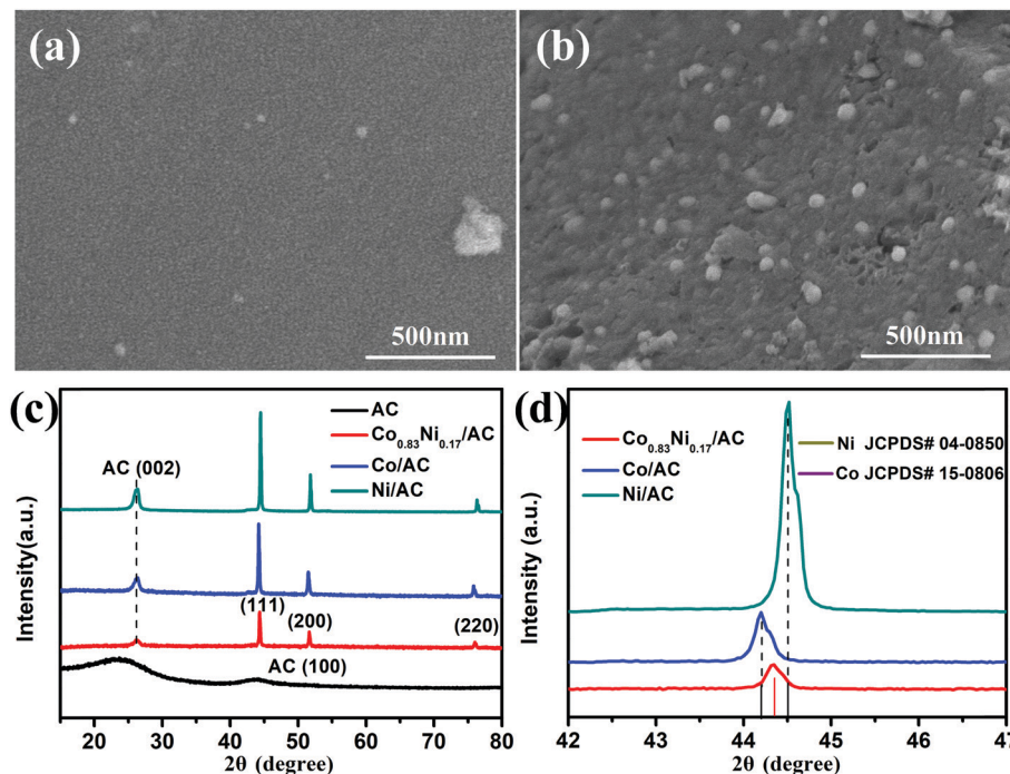
Fig. 1 Surface SEM images of (a) bare AC and (b) Co 0.83 Ni 0.17 /AC. XRD patterns (c and d) of AC, Co/AC, Ni/AC and Co 0.83 Ni 0.17 /AC samples.
