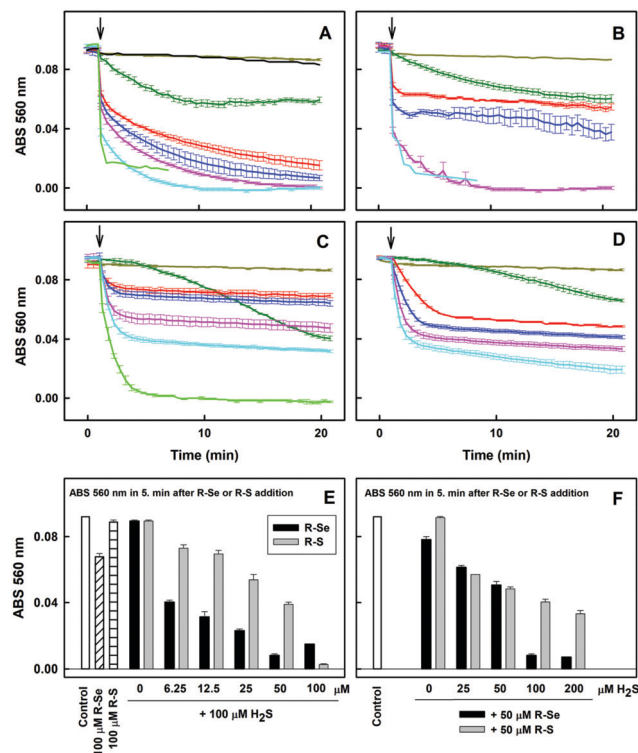
Fig. 6 The effect of R-Se and R-S on the kinetics of \cdot cPTIO reduction in the absence and presence of H 2 S. (A) The effect of R-Se and R-OH on the time-dependent reduction of \cdot cPTIO/H 2 S. Kinetics of changes in absorbance at 560 nm of 100 \mu M \cdot cPTIO after addition (indicated by an arrow) of 100 \mu M R-Se alone (dark green) and compared to the addition of 0 (dark yellow), 6.25 (red), 12.5 (blue), 25 (pink), 50 (cyan) and 100 \mu M (green) R-Se to \cdot cPTIO/H 2 S (100/100 \mu M/ \mu M). 50 \mu M R-OH added to \cdot cPTIO/H 2 S (black; 100/100 \mu M/ \mu M). Data were collected from UV-vis spectra every 30 s for 20 min. (B) The effect of H 2 S on the kinetics of reduction of \cdot cPTIO in the presence of R-Se. Kinetics of changes in absorbance at 560 nm of 100 \mu M \cdot cPTIO after addition (indicated by an arrow) of 100 \mu M H 2 S alone (dark yellow) and after addition of 50 \mu M R-Se to 0 \mu M (dark green), 25 \mu M (red), 50 \mu M (blue), 100 \mu M (pink) and 200 \mu M H 2 S (cyan). (C) The effect of R-S on the kinetics of \cdot cPTIO reduction in the presence of H 2 S. Kinetics of changes in absorbance at 560 nm of 100 \mu M \cdot cPTIO after addition (indicated by an arrow) of 100 \mu M R-S alone (dark green) and compared to the addition of 0 (dark yellow), 6.25 (red), 12.5 (blue), 25 (pink), 50 (cyan) and 100 \mu M (green) R-S to \cdot cPTIO/H 2 S (100/100 \mu M/ \mu M). (D) The effect of H 2 S on the kinetics of \cdot cPTIO reduction in the presence of R-S. Kinetics of changes in absorbance at 560 nm of 100 \mu M \cdot cPTIO after addition (indicated by an arrow) of 100 \mu M H 2 S alone (dark yellow) and after addition of 50 \mu M R-S to 0 \mu M (dark green), 25 \mu M H 2 S (red), 50 \mu M (blue), 100 \mu M (pink) and 200 \mu M H 2 S (cyan). (E) Comparison of the potency of R-Se and R-S to reduce \cdot cPTIO in the presence of H 2 S. Reduction of \cdot cPTIO (100 \mu M) by R-Se and R-S (100 \mu M) and reduction of \cdot cPTIO in the presence of H 2 S (100 \mu M) after addition of 0, 6.12, 12.5, 25, 50 and 100 \mu M R-Se or R-S. The changes in absorbance at 560 nm of 100 \mu M \cdot cPTIO were taken from (A and C) at the 5th min after the addition of the compound. (F) Comparison of the potency of R-Se and R-S to reduce \cdot cPTIO in the presence of different concentrations of H 2 S. Reduction of \cdot cPTIO (100 \mu M) by R-Se and R-S (50 \mu M) in the presence of 0, 25, 50, 100 and 200 \mu M H 2 S. The changes in absorbance at 560 nm of 100 \mu M \cdot cPTIO were taken from (B and D) at the 5th min after the addition of the compound. Mean \pm SEM, n = 2-4 .
