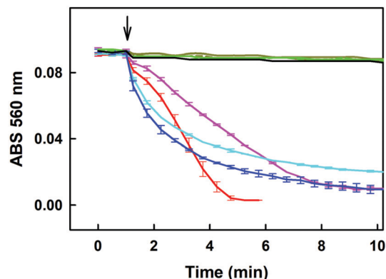
Fig. 7 Effect of GSH on the \cdot cPTIO reduction kinetics in the presence of R-Se, R-S, R-O and R-OH. Kinetics of the changes in absorbance at 560 nm of 100 \mu M \cdot cPTIO after addition (indicated by an arrow) of 100 (dashed dark-yellow) and 500 \mu M GSH (solid dark yellow); after addition of 50 \mu M R-Se to \cdot cPTIO/GSH (100/200 \mu M/ \mu M; pink), and to \cdot cPTIO/GSH (100/500 \mu M/ \mu M; red); after addition of 50 \mu M R-S to \cdot cPTIO/GSH (100/200 \mu M/ \mu M; cyan), and to \cdot cPTIO/GSH (100/500 \mu M/ \mu M; blue); after addition of 50 \mu M R-O to \cdot cPTIO/GSH (100/200 \mu M/ \mu M; dashed green), and to \cdot cPTIO/GSH (100/500 \mu M/ \mu M; solid green); and after addition of 50 \mu M R-OH to \cdot cPTIO/GSH (100/500 \mu M/ \mu M; black). Mean \pm SEM, n = 2-3 .
