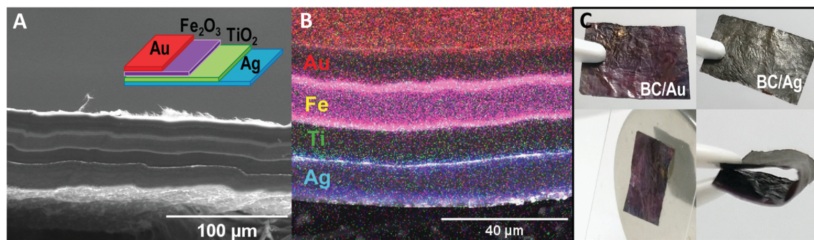
Fig. 5 (A) Millefeuille scheme of one of the possible configurations and SEM image of the cross section with the four layers of similar thicknesses visible due to the different contrasts of the nanoparticles. (B) EDX scan confirming the confined location of the different nanoparticles. (C) Upper panels: Millefeuille construct (1 cm \times 1.5 cm) showing the two exterior, Au and Ag, layers. Lower panel: The millefeuille responding to a FeNdB permanent magnet (3 cm of diameter \times 8 mm width) and the folded film without any apparent signs of mechanical failure.
