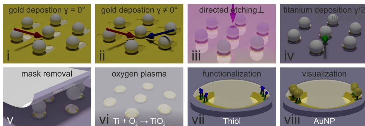
Fig. 2 Fabrication of arrays of site-specific functionalized nanocrescents. i) A thin layer of titanium (1 nm, as adhesion promoter) and gold (20 nm) are evaporated at an angle of 30^\circ with respect to the surface normal (red arrow) to deposit gold underneath the masking particles. ii) A second layer of gold is deposited at a different azimuthal angle \gamma , indicated by the blue arrows in the cartoon. This angle defines the overlap of the gold layers underneath the particle, and by this increases the contour of the crescent. iii) Reactive ion etching along the surface normal (pink arrow) is used to remove material not covered by the shadow of the particle. iv) Evaporation of a thin layer of titanium (5 nm) at half the previous azimuthal angle ( \gamma/2 ) to passivate the central area of the crescent. The deposition of titanium with an azimuthal angle in between the two gold azimuthal angles (green arrow) ensures that the tips of the crescent remain uncovered. v) Removal of the particle mask using adhesive tape. vi) Oxidation of titanium to titania and removal of residuals of the particle mask by oxygen plasma vii) Selective functionalization of the uncovered region using thiol chemistry viii) Site-selective deposition by electrostatic attraction of negatively charged gold nanoparticles onto the tip region functionalized with positively charged cysteamine molecules.
