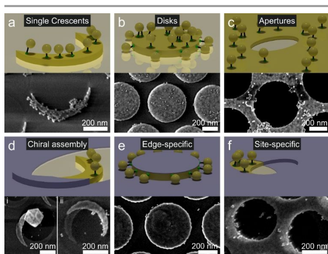
Fig. 5 Site-specific functionalization of different surface nanostructures made by colloidal lithography. a-c) Unspecific functionalization with thiols uniformly deposits gold nanoparticles onto the entire surface of the nanostructure, exemplarily demonstrated for a) single nanocrescents, b) nanodisks, and c) nanoholes. d-f) Modification of the fabrication process by adding a passivation layer under a different deposition angle selectively uncovers specific parts of the nanostructure and provides a tool to direct the deposition of the nanoparticles onto predefined areas. d) Rotated evaporation of the passivation layer selectively blocks one tip of a nanocrescent, enabling the formation of structures with a chiral character upon selective adsorption of nanoparticles. e) Direct evaporation of the passivation layer onto nanodisks blocks the top surface and allows selective functionalization of the edge of the disc. f) Azimuthal rotation of the passivation layer on top of a gold nanohole arrays enables an asymmetric functionalization of the array with AuNPs.
