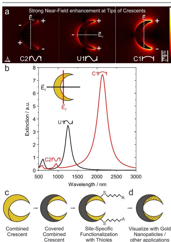
Fig. 1 Strategy for site-specific functionalization of the hotspot regions of gold nanocrescents. a) Nanocrescents are analogues of split-ring resonators and can evoke the fundamental dipole resonance (C1), the first order resonance (U1) and the second order resonance (C2). A common feature for all of these resonances is the enhanced electric field (hot spot) around their tips. b) A typical extinction spectra is given for the two polarizations. For the C polarization, the electric field is parallel to the long axis of a crescent, which reads as a C. In 90° tilted case the electric field is along the short axis of a crescent, which now reads as a U. c) Conventional functionalization chemistry would address the entire surface of the gold nanostructure. Selective functionalization of the tips can be achieved by multiple deposition steps starting with a combined nanocrescent. Subsequently, the nanocrescent can be partly covered by evaporating a blocking layer. Finally, the structure can be functionalized with thiols, which exclusively bind to the free gold surface of the nanostructure. d) To visualize the successful site-specific functionalization, we electrostatically adsorb gold nanoparticles, so that they can be seen in conventional electron microscopes.
