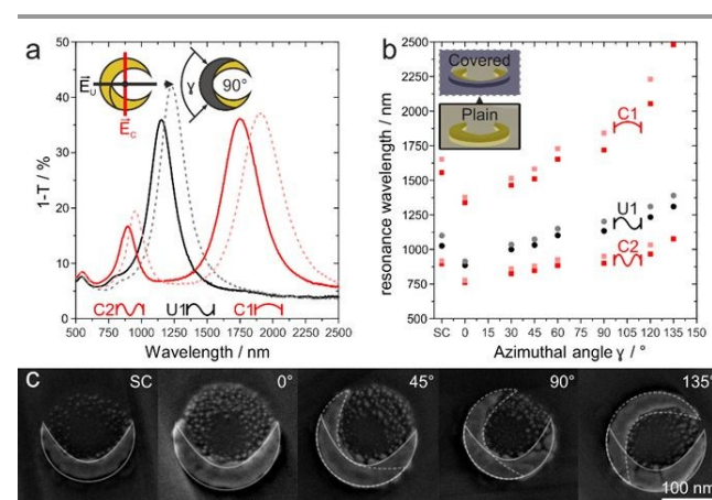
Fig. 3 Optical properties response of combined and passivated nanocrescents with different azimuthal angles \gamma . a) In the case of combined nanocrescent with \gamma = 90^\circ (solid line), linearly polarized light along the long-axis excites the fundamental resonance (C1) at around 1720 nm and the second-order resonance (C2) at around 900 nm. Perpendicularly polarized light excites the first-order resonance (U1) at around 1134 nm. The addition of a passivation layer (5 nm titanium, plasma oxidized to titania) leads to redshifts for all three resonances (dashed lines). b) The resonance behavior of an array of combined nanocrescents produced from the same colloidal mask can simply be tuned by varying the azimuthal angle \gamma between the evaporation steps. Increasing azimuthal angles increase the contour and leads to a redshift of the resonances (dark filled). The presence of the passivation layer is evidenced by a further redshift of all resonances (shaded filled). c) High magnification SEM images show the single and the combined nanocrescents made from the same colloidal mask with increasing azimuthal angle \gamma varying from 0^\circ to 135^\circ . The contour of the individual deposition steps is outlined in white color for clarity. More SEM images can be found in Figure S1.
