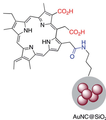
Fig. 5 A gold-silica core-shell nanocluster modified with a porphyrin based photosensitizer.
