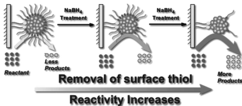
Fig. 7 Illustration of enhanced catalytic activity in a selective oxidation reaction with supported thiolate-stabilized \text{Au}_{25}(\text{SR})_{18} cluster catalysts by mild chemical stripping of their surface ligands with \text{NaBH}_4 . Reprinted with permission from ref. 82. Copyright 2014 John Wiley and Sons.
