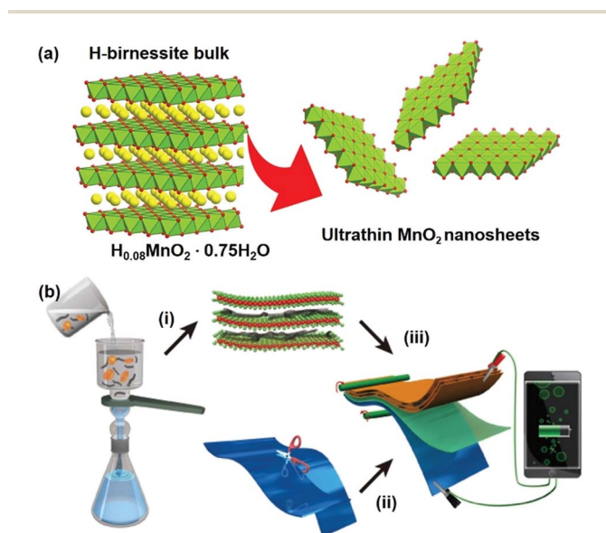
Fig. 1 (a) Crystal structure evolution by liquid exfoliation of the H-birnessite bulk into single-atomic layers. (b) Schematic illustration of (i) the vacuum-assisted filtration strategy to fabricate the freestanding MnO 2 /MWCNT hybrid membrane; (ii) trimmed zinc foil as the anode material; (iii) assembly of a proof-of-concept paper-like ZIB.
