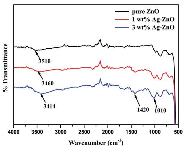
Fig. 5 FT-IR spectra of bare ZnO NPs and 1 and 3 wt% Ag–ZnO nanocomposites.
