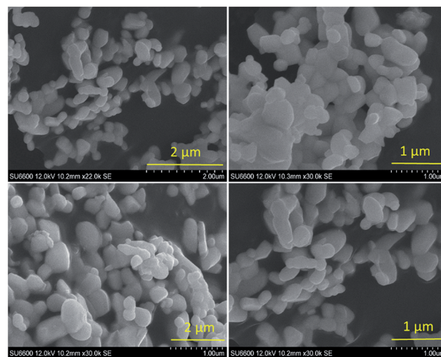
Fig. 3 SEM images of \text{U}_3\text{O}_8/\text{ZnO} nanocomposite.
