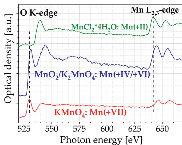
Fig. 5 Oxygen K-edge and manganese \text{L}_{2,3} -edge spectra of manganese dichloride ( \text{MnCl}_2 \cdot 4\text{H}_2\text{O} ), manganese oxide/potassium manganate ( \text{MnO}_2/\text{K}_2\text{MnO}_4 ), and potassium permanganate ( \text{KMnO}_4 ) (accumulated over 10 000 pulses). For better visibility the spectra are shifted along the y-axis.
