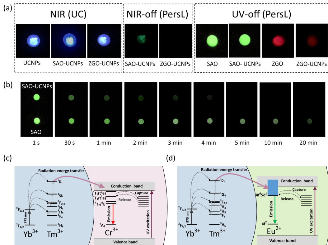
Fig. 5 (a) Emission of \text{LiYbF}_4:0.5\%\text{Tm}^{3+}@ \text{LiYF}_4 (UCNPs), \text{SrAl}_2\text{O}_4:1\%\text{Eu}^{2+}, 0.5\%\text{Dy}^{3+} (SAO), \text{SrAl}_2\text{O}_4:1\%\text{Eu}^{2+}, 0.5\%\text{Dy}^{3+} -UCNPs (SAO-UCNPs), \text{ZnGa}_2\text{O}_4:0.5\%\text{Cr}^{3+} (ZGO) and the composite \text{ZnGa}_2\text{O}_4:0.5\%\text{Cr}^{3+} -UCNPs (ZGO-UCNPs) under NIR excitation and after (PersL) NIR or UV excitation. (b) Persistent luminescence of SAO and SAO-UCNPs after irradiation with UV light. The photos were taken using an iPhone 13 camera. (c) and (d) Simplified mechanisms of the observed upconversion and persistent luminescence, showing radiation energy transfer between UCNPs and (c) ZGO or (d) SAO components of composite materials.
