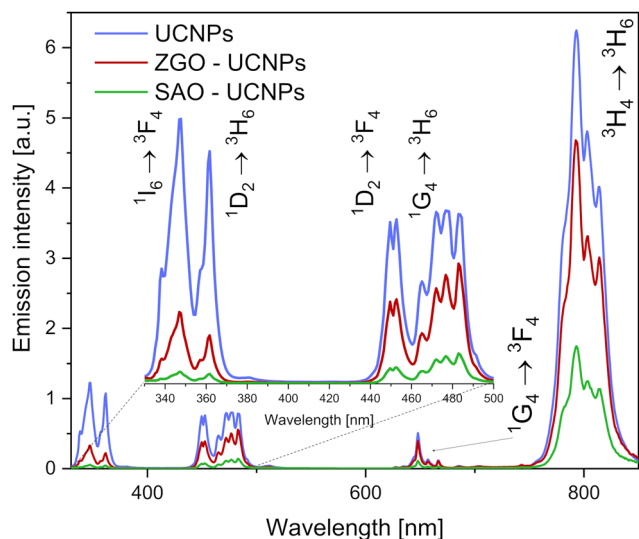
Fig. 4 Emission spectra of the \text{LiYbF}_4:0.5\%\text{Tm}^{3+}@ \text{LiYF}_4 (UCNPs), \text{ZnGa}_2\text{O}_4:0.5\%\text{Cr}^{3+} -UCNPs (ZGO-UCNPs) and \text{SrAl}_2\text{O}_4:1\%\text{Eu}^{2+}, 0.5\%\text{Dy}^{3+} -UCNPs (SAO-UCNPs) materials under 975 nm laser excitation with a power density of 6 \text{ W cm}^{-2} .
