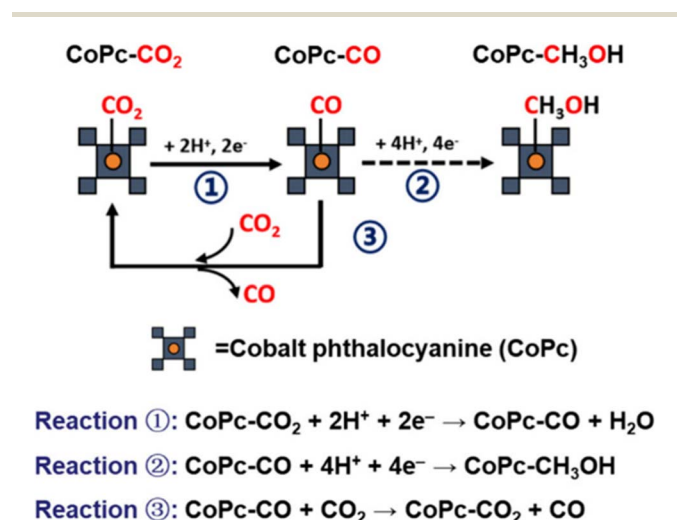
Fig. 4 Schematic illustration of the CO 2 /CO competitive binding mechanism on CoPc. Reaction (1) represents the reduction of CO 2 to CO. Reaction (2) is the further reduction from CO to CH 3 OH. Reaction (3) is the competitive displacement of CO by CO 2 . 73 Reproduced from ref. 73 with permission from American Chemical Society, copyright 2024.
