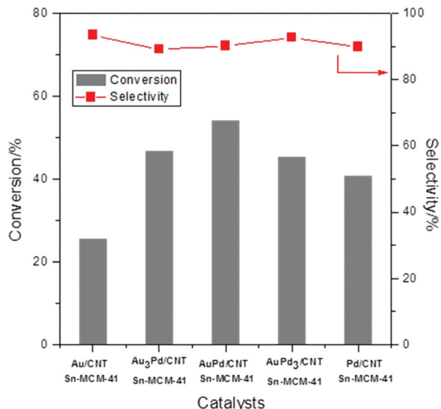
Fig. 4 Performance of the catalytic system consisting of mono- or bimetallic Au–Pd on unmodified CNTs (with different Au/Pd values) and Sn-MCM-41-XS. Reaction conditions: 0.25 M glycerol in 20 ml methanol; 0.1 g of AuPd/CNTs; 0.2 g of Sn-MCM-41-XS; 140 °C; 30 bar pressure; 4.5 h batch time.
