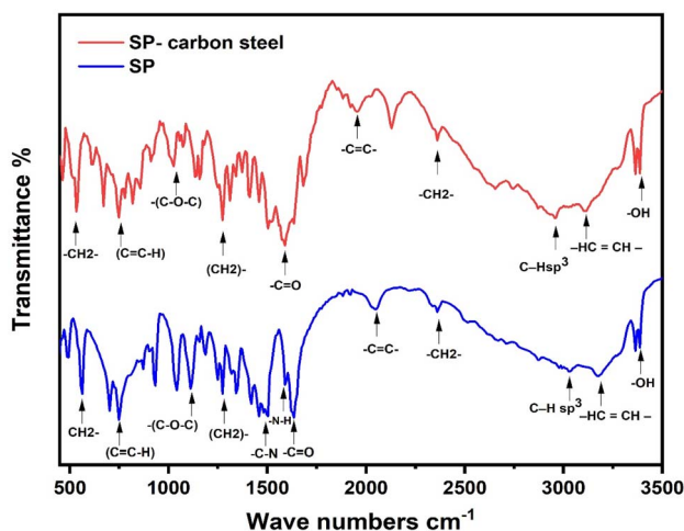
Fig. 11 ATR-FTIR spectrum of SP inhibitor on the carbon steel surface after immersion for 24 h in 0.5 N HCl with the optimum concentration of 2.5 g L -1 of SP inhibitor.
