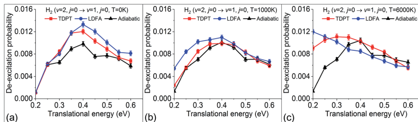
Fig. 7 Vibrational deexcitation probabilities from H_2 ( v=2, j=0 ) to H_2 ( v=1, j=0 ) simulated by MD, MDEF(LDFA), and MDEF(TDPT), with electronic temperatures of 0 K (a), 1000 K (b), and 6000 K (c).
