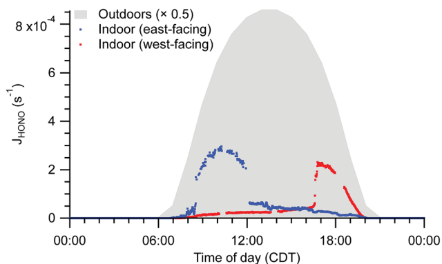
Fig. 5 Indoor photolysis rate constants of HONO calculated from solar spectral photon fluxes measured near the east-facing and west-facing windows under clear sky conditions. Photon fluxes were determined from measured spectral irradiance. Outdoor HONO photolysis rate constants based on tropospheric ultraviolet and visible (TUV) radiation model results are shaded in grey for comparison. 64
