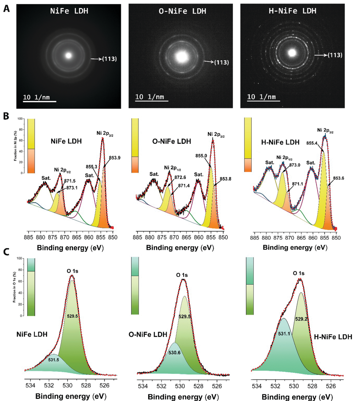
Fig. 3 Material characterization. (A) SAED patterns of NiFe LDH, O-NiFe LDH and H-NiFe LDH. High-resolution XPS spectra of (B) Ni 2p and (C) O 1s of NiFe based catalysts before (NiFe LDH) and after 100 hours of HER (H-NiFe LDH) and OER (O-NiFe LDH) testing. The color columns show the peak area integration ratio of the corresponding species.
