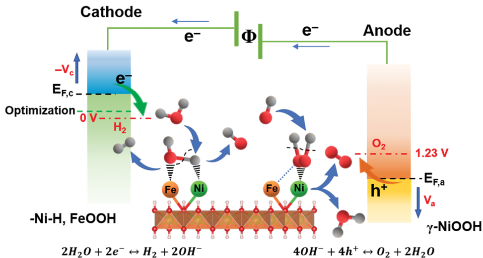
Fig. 6 Schematic representation of the electrocatalytic generation of \text{H}_2 in alkaline media. \text{FeOOH} and \text{Ni-H} are the formed surface adsorbed intermediates during HER process, while, \gamma\text{-NiOOH} is the observed surface intermediate under OER process. The self-optimized bifunctional electrocatalyst NiFe LDH reduces the required driving energy and thus realizes a highly versatile energy conversion efficiency.
