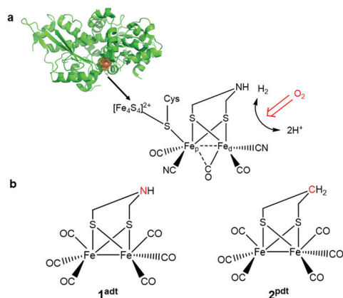
Fig. 1 (a) A schematic representation of the [FeFe] hydrogenase from Chlamydomonas reinhardtii (Cr HydA1, PDBID: 3LX4) and the H-cluster. (b) The two biomimetic complexes, 1 adt and 2 pdt , used to investigate reactivity towards O 2 and ROS.
