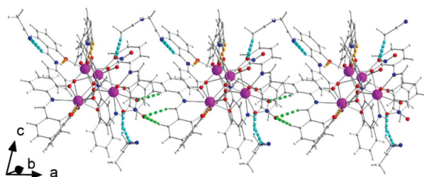
Fig. 4 A portion of a chain of tetranuclear cluster and MeCN molecules parallel to the a crystallographic axis in the crystal structure of 1.4MeCN. Dashed orange lines indicate intramolecular N-H\cdots O bonds within the LH^- ligands and dashed cyan lines indicate H bonds involving the lattice MeCN molecules; dashed light green lines represent the H bonds that are responsible for the formation of chains.
