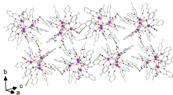
Fig. 6 A part of a layer parallel to the (-101) plane formed as a result of C-H\cdots O H bonds (dashed light green lines) between the tetranuclear cluster molecules in the crystal structure of 2.2.4MeCN, see the text for details. Only the H atoms involved in H bonds that contribute to the layer formation are shown.
