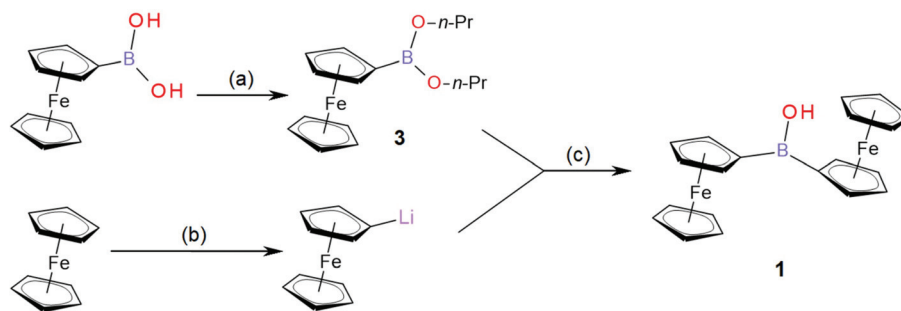
Fig. 1 Synthesis of Fc 2 BOH (1); (a) in toluene, excess of n -propanol, molecular sieve 4 Å, 1 h azeotropic dehydration; (b) in THF under inert atmosphere, 1 mol. eq. of t -BuLi, 0 °C, 15 min; (c) in THF under inert atmosphere, 0 °C, 15 min, H 2 O quenching, further extraction and purification according to experimental details in section 2.3.
