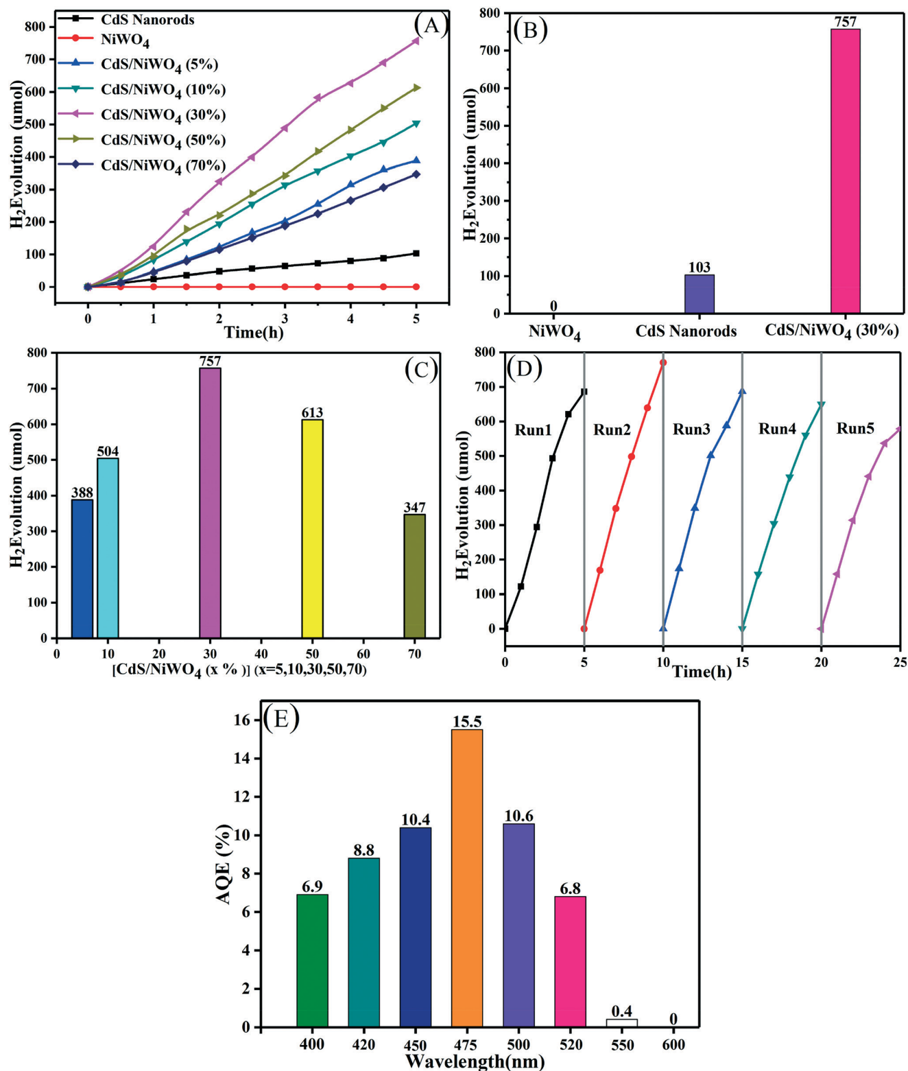
Fig. 7 (A–C) The \text{H}_2 production activity curves of CdS nanorods, \text{NiWO}_4 and [\text{CdS/NiWO}_4 (x%)] (x = 5, 10, 30, 50, 70) in 30 ml 10% lactic acid solution; (D) stability test on the [\text{CdS/NiWO}_4 (30%)] sample; (E) the AQE of the [\text{CdS/NiWO}_4 (30%)] sample in 30 ml 10% lactic acid solution.
