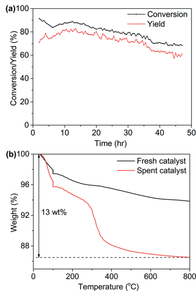
Fig. 6 (a) Stability test for Ni/Al 2 O 3 -PD catalyst. 1-Hexanol at 1 \mu\text{L min}^{-1} with 8 \text{mL min}^{-1} NH 3 and 20 \text{mL min}^{-1} N 2 flowed through 200 mg catalyst at 230 °C. GHSV = 1.12 \times 10^4 \text{ h}^{-1} . (b) TG analysis for Ni/Al 2 O 3 -DP catalyst before and after reaction.
