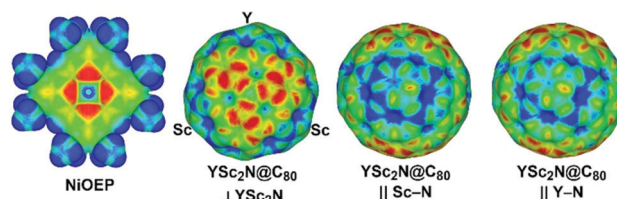
Fig. 3 Electrostatic potentials in Ni(OEP) and \text{YSc}_2\text{N}@C_{80} molecules (red and blue indicate more negative and positive potentials, respectively) mapped on the electron density isosurface of 0.01 a.u. \text{YSc}_2\text{N}@C_{80} is shown in three orientations: normal to the \text{YSc}_2\text{N} plane and along the Sc–N and Y–N bonds.
