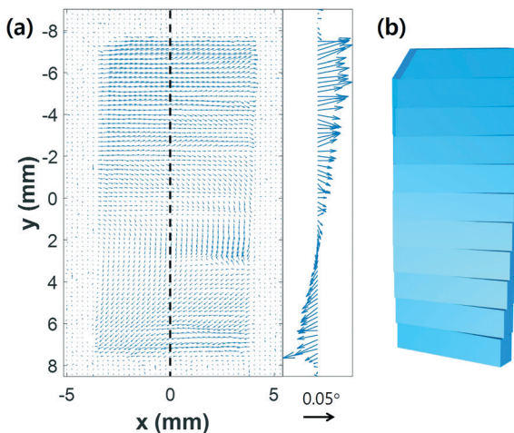
Fig. 3 Vector plot of domain bending directions evaluated from \Delta\theta at two different azimuthal angles are shown (a). Line profile along the dashed line in the left figure on the right side represents the twisted lattice. Lattice-plane twisting and stripe patterns parallel to [0001] direction over the epitaxial layer is shown (b).
