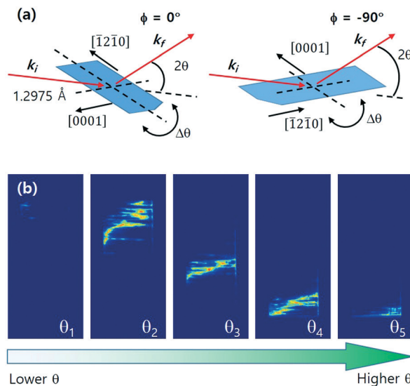
Fig. 1 Experimental configurations for X-ray diffraction topography of GaN ( 10\bar{1}0 ) at different azimuthal angles (a). At a 10\bar{1}0 Bragg angle of 27.8^\circ , the flat panel sensor was set parallel to sample. Partially diffracted images were obtained at various incident angles to reconstruct the rocking curve and FWHM images. Partially diffracted images at various incident X-ray angles (b).
