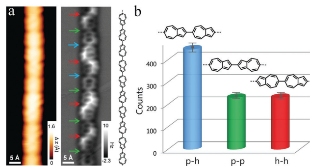
Fig. 2 (a) High-resolution STM image of a 2,6-polyazulene chain ( V_s = -0.1 V, I_t = 0.3 nA) and the corresponding nc-AFM image ( V_s = -5 mV, Oscillation amplitude: \sim 80 pm). The pentagon–heptagon (p–h), pentagon–pentagon (p–p) and heptagon–heptagon (h–h) linkages are indicated by blue, green and red arrows, respectively. The corresponding chemical model of the chain is also shown. (b) Statistical analysis of the different linkages within the polymers.
