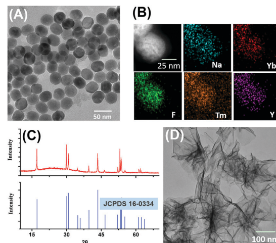
Fig. 1 TEM (A), EDS mapping (B) and X-ray diffraction (XRD) patterns (C) of NaYF 4 :Yb,Tm UCNP; (D) TEM of MnO 2 nanosheets.
