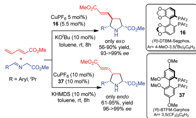
Scheme 17 \text{Cu}^I/\text{DTBM-Segphos} catalyzed 1,3-dipolar cycloaddition of azomethine ylides and 1,3-dienes.
