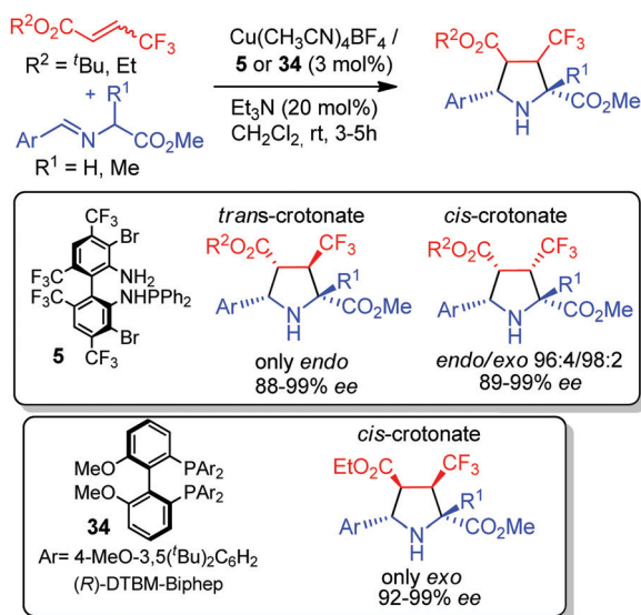
Scheme 15 \text{Cu}^I/(\text{S})\text{-TF-BiphamPhos} catalyzed cycloaddition with trifluorocrotonates.
