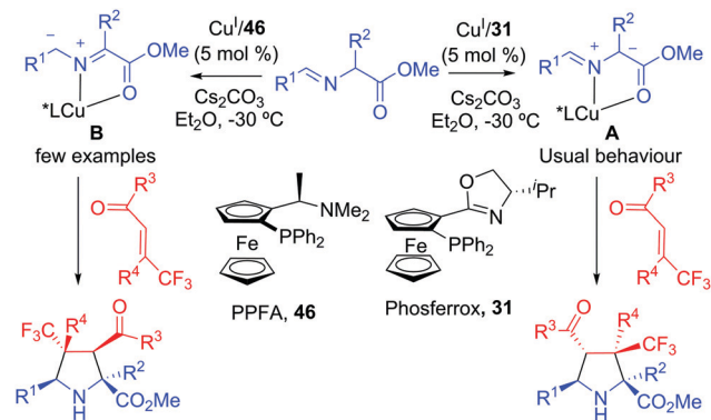
Scheme 28 Cu I -Catalyzed regiodivergent 1,3-dipolar cycloaddition of iminoesters with \beta -trifluoromethyl enones.
