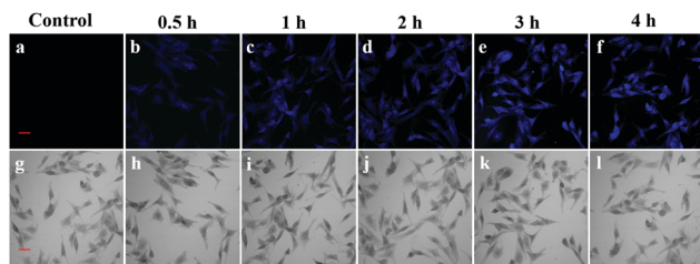
Fig. 3 Confocal fluorescence images of TYR in B16 cells at different times. (a) B16 cells only (control). Then the B16 cells were incubated with 10 μM probe 1 for (b) 0.5 h, (c) 1 h, (d) 2 h, (e) 3 h, and (f) 4 h. The differential interference contrast (DIC) images of the corresponding samples are shown below (panels g–l). Scale bar: 20 μm.
