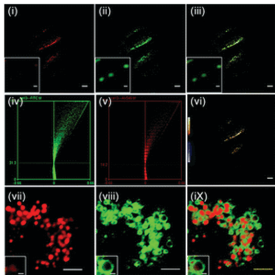
Fig. 65 Probe 44 colocalization assay in HeLa cells. Cells treated with "MPO-44" for 12 h and then H_2O_2 for half an hour were stained with LysoTracker Green DND-26 for half an hour: (i) fluorescence image of "MPO-44"; (ii) fluorescence image of LysoTracker Green DND-26; (iii) merged image of (i) and (ii); ICA scatter plots of "MPO-44" (iv) and LysoTracker Green DND-26 (v); (vi) PDM image. The PDM scale bar is inserted. Cells expressing LAMP2-EGFP were treated with "MPO-44" for 12 h and then H_2O_2 for half an hour. (vii) Fluorescence image of "MPO-44"; (viii) image of LAMP2-EGFP; (ix) merged image of "MPO-44" and LAMP2-EGFP. The scale bar is 10 \mu m in original pictures, 1 \mu m in amplified pictures. Copyright 2013 Royal Society of Chemistry.
