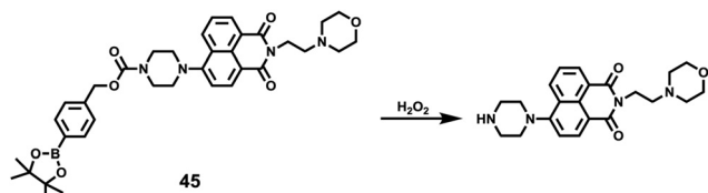
Scheme 34 Fluorescent probe 45 for H_2O_2 .
