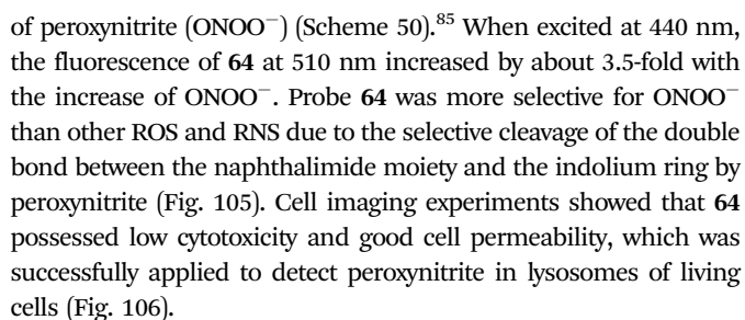
Scheme 50 Fluorescent probe 64 for ONOO - .
