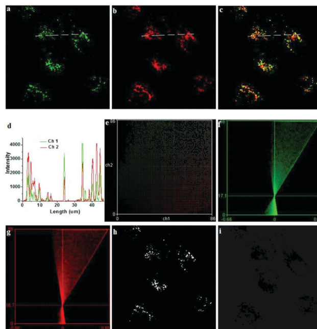
Fig. 103 63 co-localizes to lysosomes in MCF-7 cells. MCF-7 was stained with (a) 5.0 \mu M 63 with NO solution (20 \mu M) for 5 min at 37 ^{\circ} C (Channel 1: \lambda_{\text{ex}} = 840 nm, \lambda_{\text{em}} = 520–560 nm) and (b) 5.0 \mu M NR (Channel 2: \lambda_{\text{ex}} = 559 nm, \lambda_{\text{em}} = 565–610 nm). (c) Overlay of (a) and (b). (d) Intensity profile of regions of interest (ROI) across MCF-7 cells. (e) Intensity correlation plot of stain 63 and NR. ICA plots of (f) stain 63 and (g) stain NR. PDM images with (h) positive PDM values in the pixels and (i) negative PDM values in the pixels. Copyright 2012 American Chemical Society.
