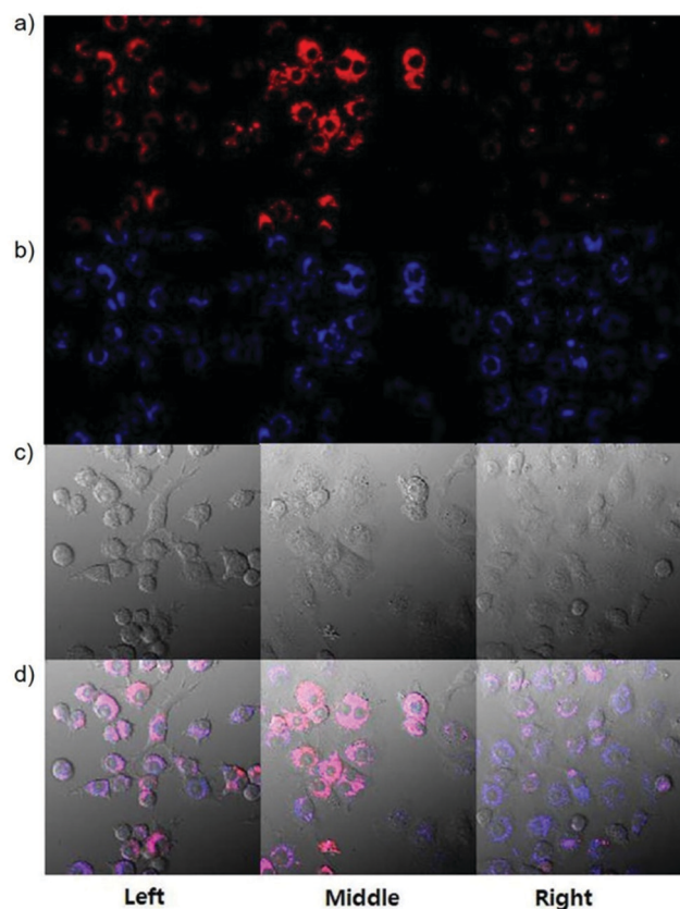
Fig. 67 Probe 45 was localized to lysosomes in RAW264.7 cells. Confocal microscopy images of probe 45 on the endogenous H_2O_2 : (a) probe 45 (red, ex405/em490–590 nm); (b) LysoTracker Blue DND-22 (blue, ex405/em430–455 nm); (c) bright field (gray); (d) overlay of (a) and (b) (purple). Left: No treatment; middle: 1 \mu g mL^{-1} PMA (Phorbol 12-myristate 13-acetate), 1 h; right: 1 \mu g mL^{-1} PMA, 1 h and 100 \mu M TEMPO (2,2,6,6-tetramethylpiperidine-1-oxyl, ROS scavenger), 1 h. (For producing endogenous H_2O_2 , the RAW264.7 cells were treated with PMA. All cells were stained with 5 \mu M probe 45 , 100 nM LysoTracker for 30 min; scale bar: 10 \mu m .) Copyright 2015 Nature.
