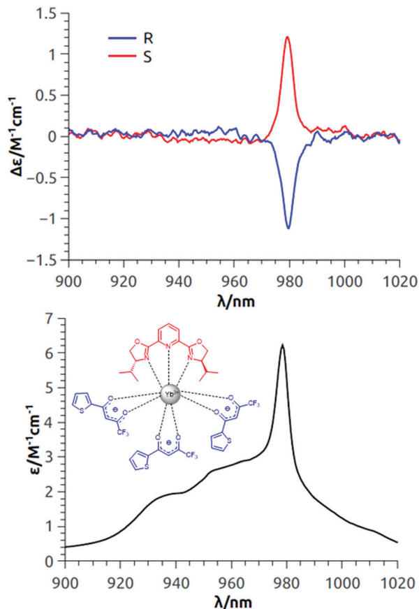
Fig. 3 Top: NIR-ECD spectra of both the enantiomers of \text{Yb}(\text{NTA})_3\text{PrPyBox} ; bottom: total NIR absorption. The spectra are measured in 7 mM \text{CH}_2\text{Cl}_2 solution (room temperature).
