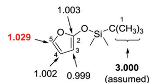
Scheme 11 Carbon isotope effects (R/R 0 ) calculated for TBSOF furan. The three methyl carbons of the tBu group (in bold) were taken as the internal standard.
