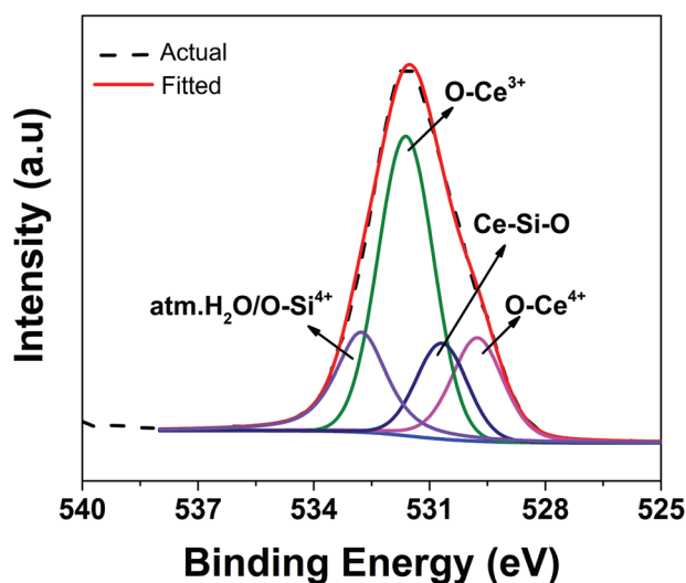
Fig. 5 (b) Deconvoluted and fitted XPS spectrum of O (1s) taken from different thickness CeOx films (b) 50 cycles.
