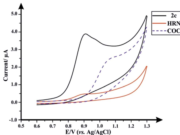
Fig. 1 Typical cyclic voltammograms obtained separately for (2c), HRN and COC; solution composition: 50 \mu\text{g mL}^{-1} of each drug within a 0.04 M B-R buffer pH 7.0; scan rate: 50 \text{mV s}^{-1} .
