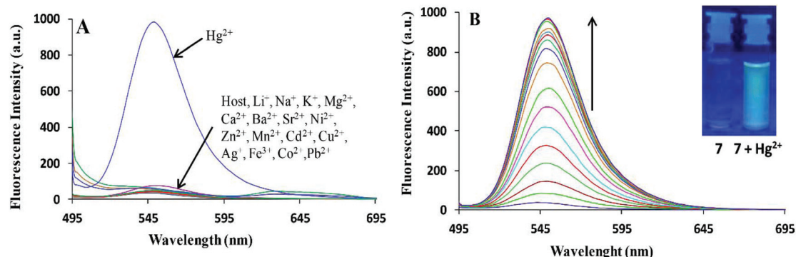
Fig. 13 (A) Changes in the fluorescence emission spectra of 195 nM solution of 12 (FON) upon the addition of 10 μM of different metal ion salts in 15 aqueous media; (B) changes in the fluorescence emission spectra of 195 nM solution of 12 (FON) upon the successive addition of 0 to 10 μM of Hg 2+ in an aqueous medium. Adapted with permission from ref. 70. Copyright 2013 the Centre National de la Recherche Scientifique (CNRS) and the Royal Society of Chemistry.
