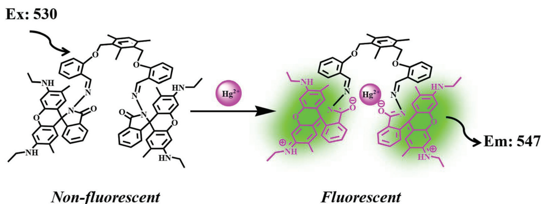
Fig. 14 Process of sensing through the coordination of Hg 2+ . Adapted with permission from ref. 70. Copyright 2013 CNRS and the Royal Society of Chemistry.
