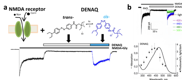
Fig. 4 (a) Schematic illustration of azobenzene-based quaternary ammonium compounds for optical control of ion channels to regulate neuronal excitability. (b) Light-controlled inhibition of NMDA receptor-mediated currents by DENAQ (adapted from ref. 132 with permission from the © 2021, American Chemistry Society).
