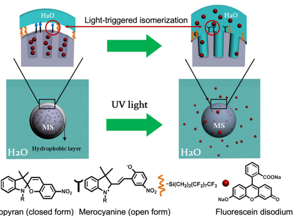
Fig. 26 The light-responsive release system involved MSNs modified with an optimal ratio of spiropyran and perfluorodecyltriethoxysilane, which rendered the particle surface hydrophobic and blocked cargo release. However, UV light at 365 nm triggered the spiropyran to convert from a "closed" to "open" form, making the surface hydrophilic and allowing the encapsulated cargo fluorescein disodium to diffuse out of the pores (adapted from ref. 240 with permission from the © 2014 American Chemical Society).
