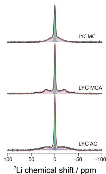
Fig. 6 7 Li static NMR spectra of MC, MCA, and AC samples and the deconvolution fits.
