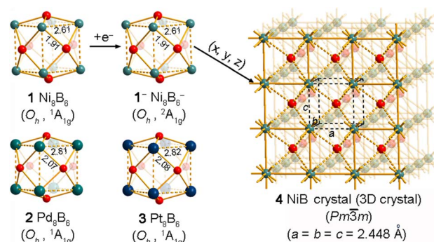
Fig. 1 Optimized structures of O_h \text{Ni}_8\text{B}_6 (1), O_h \text{Ni}_8\text{B}_6^- ( 1^- ), O_h \text{Pd}_8\text{B}_6 (2), and O_h \text{Pt}_8\text{B}_6 (3) clusters at the PBE0 level and 3D \text{NiB} (4) crystal assembled from the structural motif of \text{Ni}_8\text{B}_6 (1) at the GGA-PBE level, with the necessary bond lengths and lattice parameters indicated in Å.
