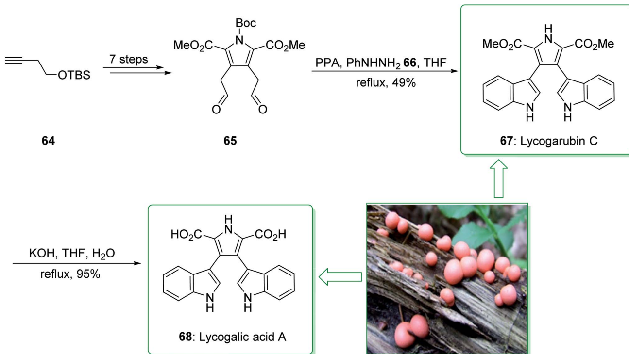
Scheme 9 Total synthesis of lycogarin C (67) and lycogalic acid (68).
