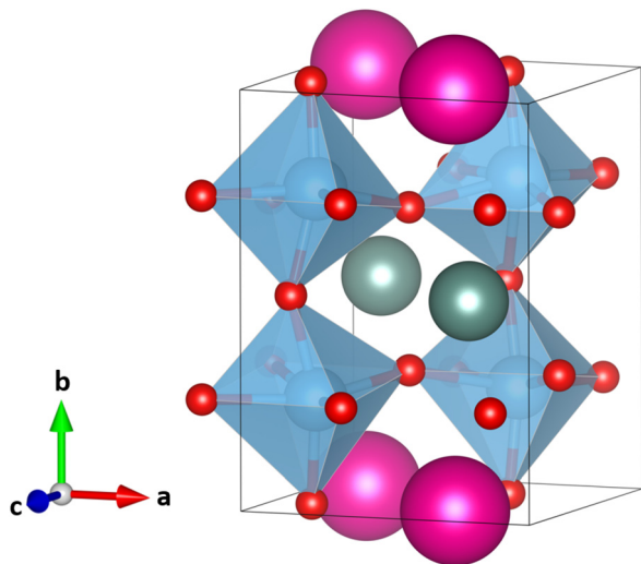
Fig. 6 Second-lowest energy perovskite-like structure of the 33 calculated YRbTi 2 O 6 structures with Y(III) cations colored in grey, Rb(I) cations in pink, Ti(IV) cations in blue, and O(–II) anions in red. In planar A-site ordering and with the tilt system a^-b^+a^- the space group is Pmc2_1 . The structure is 35 kJ mol –1 higher in energy compared to the lowest-energy structure in Fig. 5.
