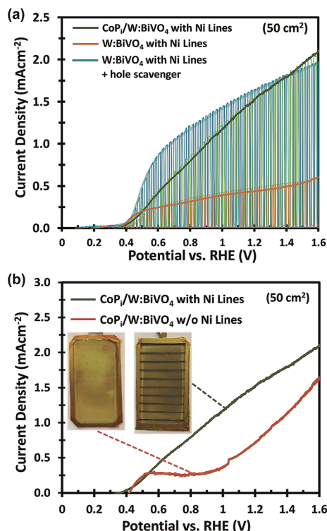
Fig. 5 (a) J - V curves under constant, dark and chopped AM 1.5G illumination comparing the performance of large area (50 cm²) W:BiVO₄ photoanodes with Ni lines, either in 2.0 M KPᵢ buffer solution with 0.5 M Na₂SO₃ (blue), or without hole scavenger, before (orange) and after (green) photo-electrodeposition of CoPi. (b) J - V curves comparing CoPi-modified W:BiVO₄ photoanodes with (green) and without (red) Ni lines measured in 2.0 M KPᵢ buffer, pH 7, under AM 1.5G illumination. Inset: photographs of the CoPi deposited on W:BiVO₄ photoanodes without (left) and with (right) Ni lines.
