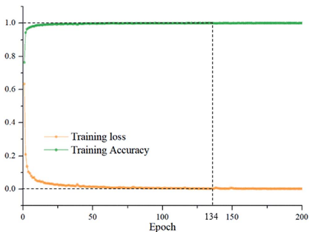
Fig. 5 The relationship between epoch and training performance.
