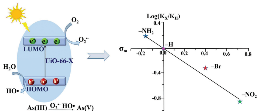
Fig. 10 Proposed mechanism (left) and Hammett plot (right) for photocatalytic oxidation of \text{As(III)} by UiO-66-X ( X = \text{H}, \text{NH}_2, \text{NO}_2 or \text{Br} ). Reproduced from ref. 43 with permission from the PCCP Owner Societies.
