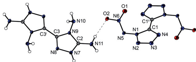
Fig. 7 Molecular unit of 8 . Ellipsoids are drawn at the 50% probability level. Selected bond lengths (Å): C1–C1' 1.443(3), C3–C3' 1.448(2), C2–N11 1.317(2). Selected torsion angles (°): N4–C1–C1'–N1' 1.7(3), N8–C3–C3'–N9' 0.2(2). Symmetry code: (i) 2 - x, 1 - y, -z (ii) -x, -y, 2 - z .
