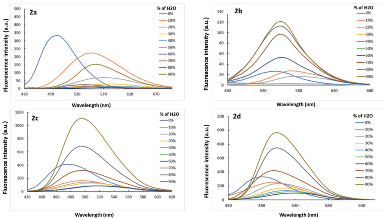
Fig. 4 Emission of dyes 2a–2d in dioxane–water mixtures with different water volume fractions ( 1 \times 10^{-5} M) at RT. Excitation wavelengths depend on \lambda_{\max} of each dioxane–water mixture as shown in the supporting information† (Fig. S1†).
