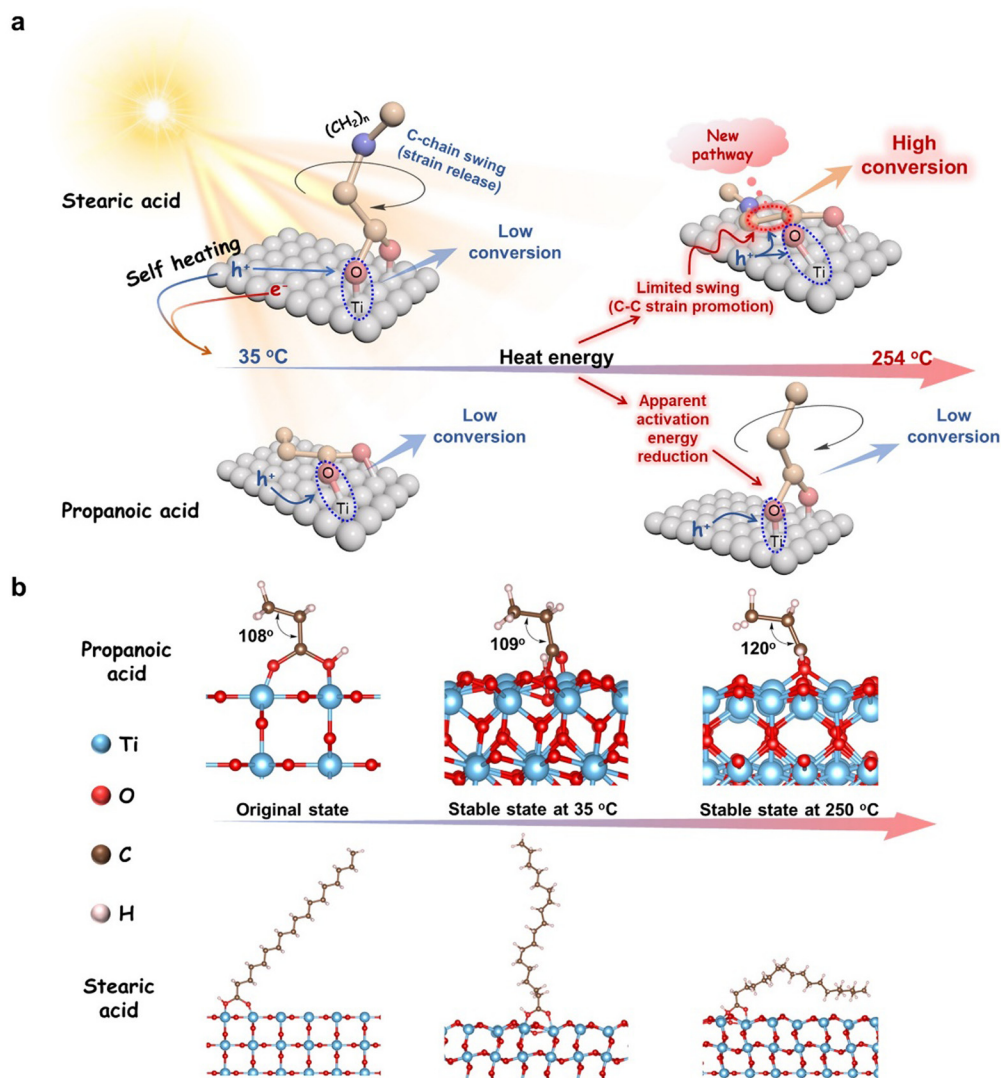
Fig. 5 Plausible reaction pathway for the photocatalytic decarboxylation of fatty acids over \text{TiO}_2 with different temperature-independent AQEs. (a) Long-chain fatty acids accumulate heat energy through shifting to attach to the surface of \text{TiO}_2 at high temperatures to enable h_{\text{vb}}^+ activation and the short-chain fatty acids undergo an upright flip at high-temperature that counteracts the enhanced high-temperature h_{\text{vb}}^+ activation over \text{TiO}_2 . (b) Theoretical calculation results showing different adsorption models of propionic acid and stearic acid on the \text{TiO}_2 surface between 35 °C and 254 °C.
