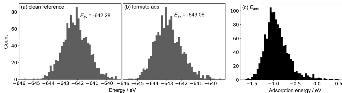
Fig. 2 Sample energy distributions for (a) clean Ga–In at 450 K (standard deviation: 0.76 eV). Note that a reference energy of E_{\text{CO}_2} + \frac{1}{2}E_{\text{H}_2} has been added to allow direct comparison to the formate-adsorbed surface. (b) The energy distribution for Ga–In with formate adsorbed to the surface at 450 K (standard deviation: 0.86 eV). (c) The adsorption energy of formate calculated by subtracting clean energies from adsorbed energies in a matching point-by-point fashion.
