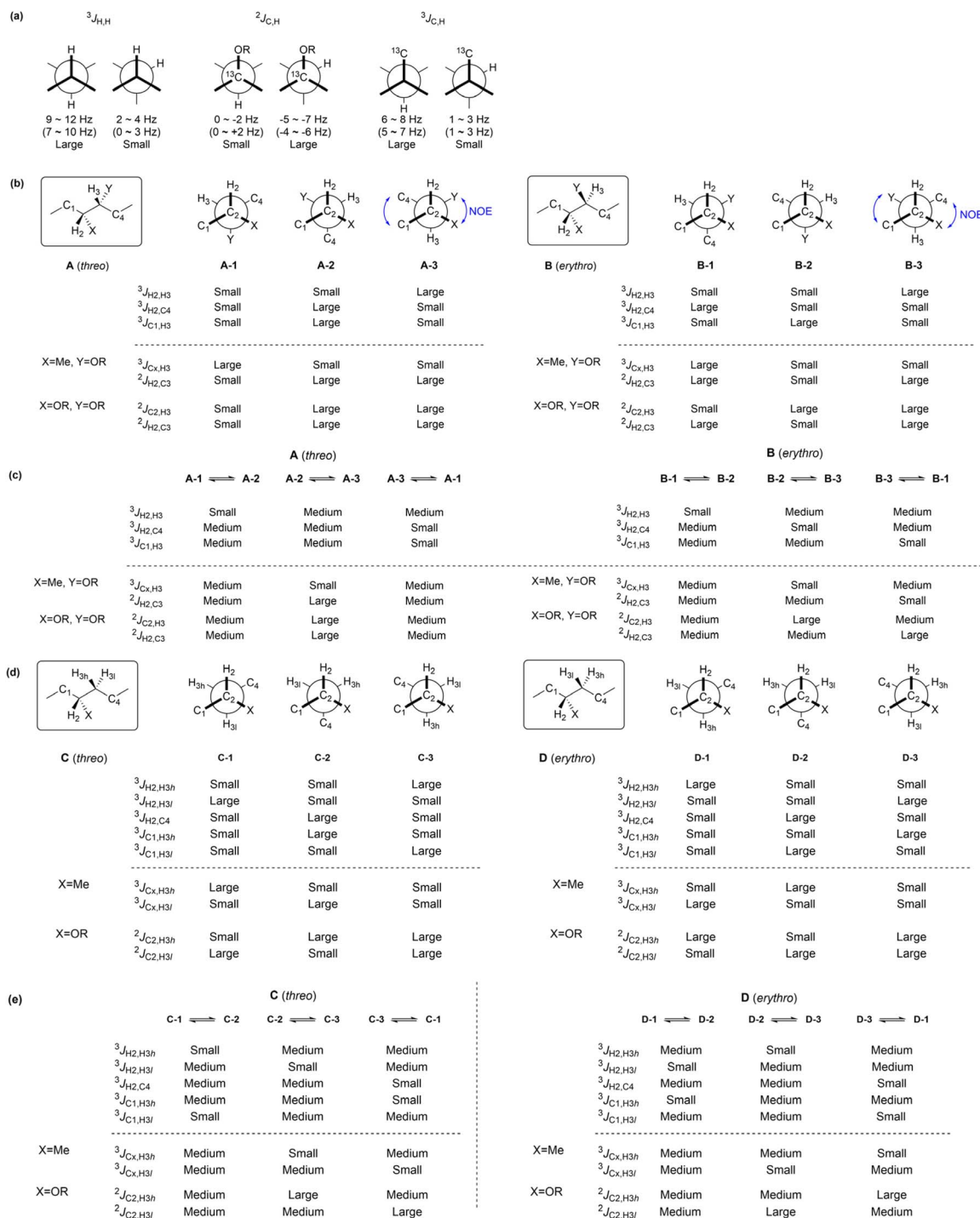
Fig. 2 Murata's JBCA strategy: (a) dihedral angle dependence of spin-coupling constants, ^3J_{H,H} and ^{2,3}J_{C,H} (values in parentheses correspond to the 1,2-dioxygenated systems. R represents H, alkyl, or acyl groups). (b) Dependence of ^3J_{H,H} and ^{2,3}J_{C,H} on the dihedral angles between vicinal methine carbons in 2,3-disubstituted butane systems. (c) Dependence of ^3J_{H,H} and ^{2,3}J_{C,H} on the dihedral angles between vicinal methine carbons in alternating butane systems. (d) Dependence of ^3J_{H,H} and ^{2,3}J_{C,H} on the dihedral angles between methine and methylene carbons in 2-substituted butane systems. (e) Dependence of ^3J_{H,H} and ^{2,3}J_{C,H} on the dihedral angles between methine and methylene carbons in alternating butane systems.
