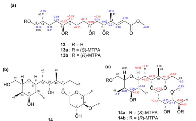
Fig. 11 (a and c) \Delta\delta_{S-R} values of MTPA esters 13a and 13b (a) and 14a and 14b (c). (b) Structure of 14 .
