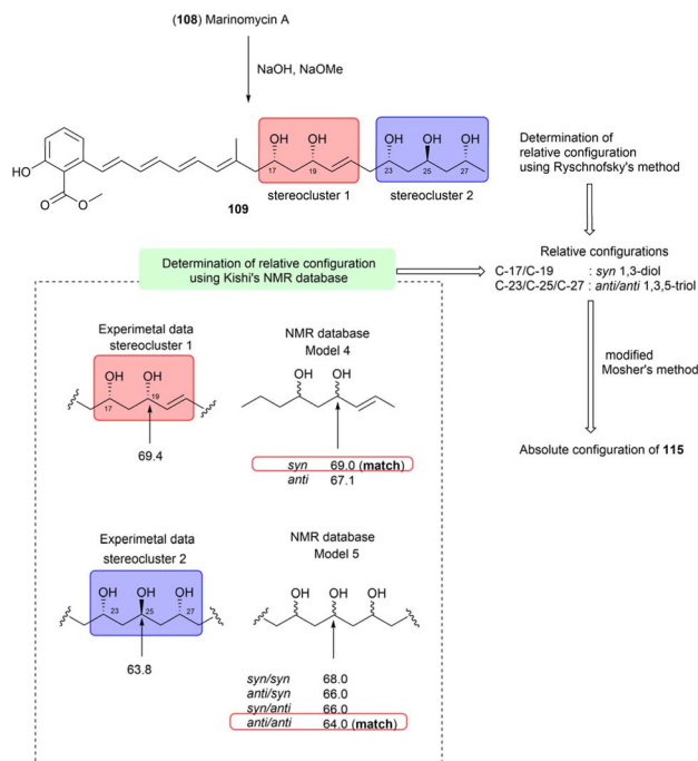
Fig. 66 Comparison of the experimental 13 C NMR data of stereocenter A in the degradation product (109) with the corresponding carbons in model 1. Data recorded in DMSO- d_6 .
