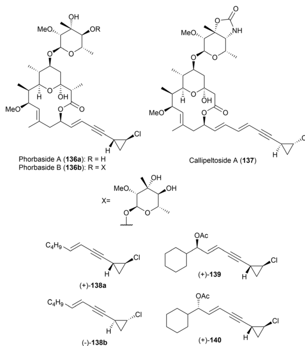
Fig. 84 Structures of (+)-phorbisides A and B (136a and 136b), (–)-callipeltoside A (137), and synthesized enantiomeric models ((+)-138a, (–)-138b, (+)-139, and (+)-140).
