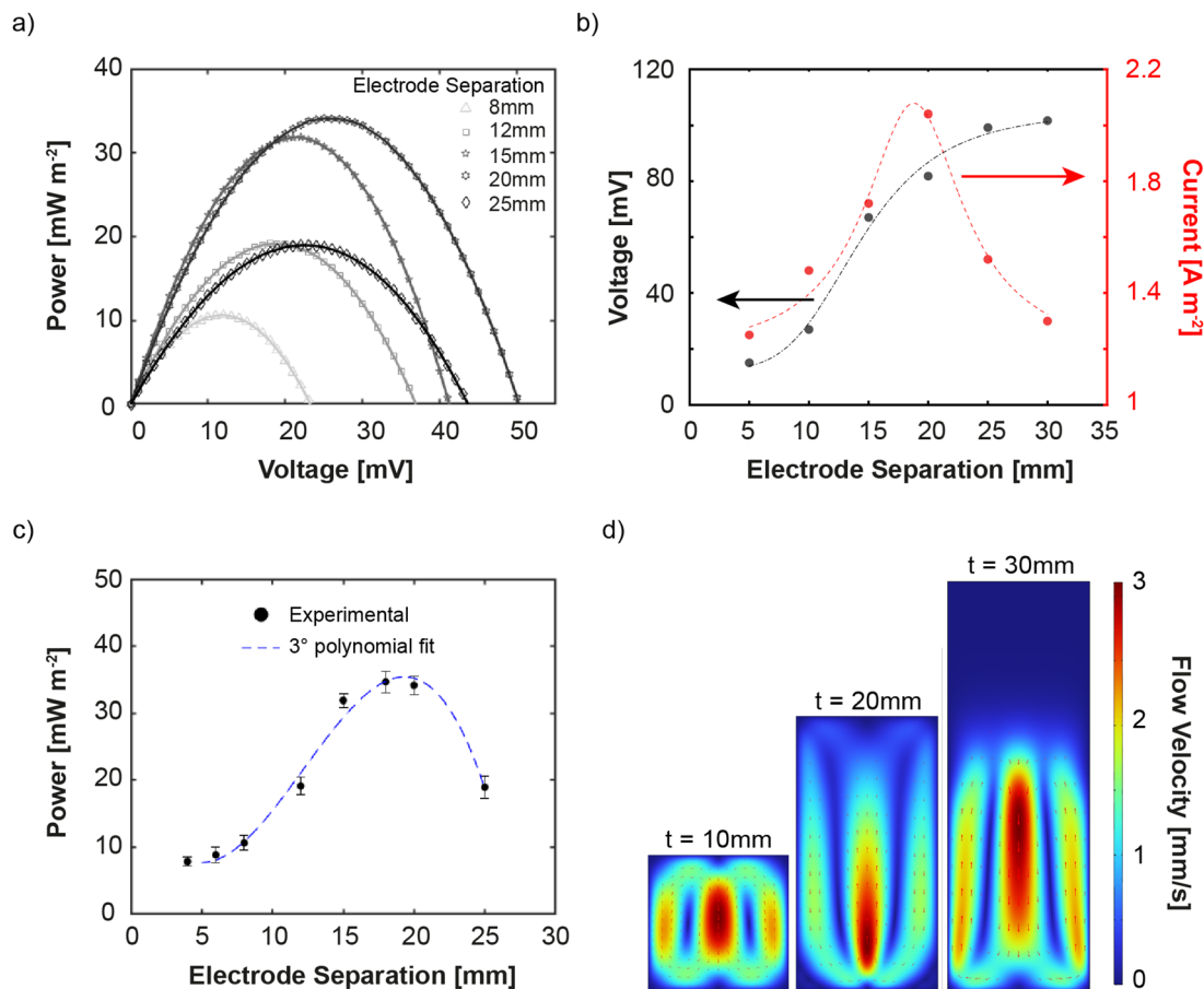
Fig. 4 (a) The output power measured experimentally for TEC cells with different electrode separation (i.e. electrolyte or hydrogel thickness) as a function of voltage. (b) V_{\text{oc}} and current density calculated with a complete COMSOL multiphysics simulation as a function of electrode separation. (c) The experimental result for the maximum output power as a function of electrode separation along with a 3rd-order polynomial fit just to underline the trend. (d) The convection velocity at the electrode/electrolyte interface obtained for cells with 10 mm width and different heights, explaining the reason for the performance decay after 20 mm (obtained from simulations).
