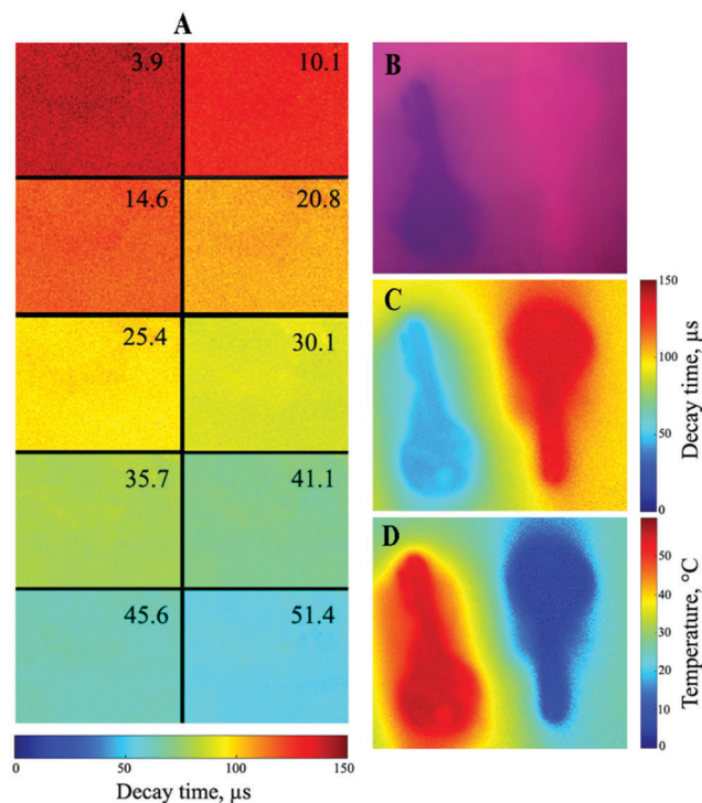
Fig. 7 Application of the Pd-1 /PVCl-PAN planar optode for lifetime imaging of temperature. (A) False color decay time images of a sensor foil with temperatures (°C) indicated in the upper right corner. (B–D) Time-resolved imaging with the help of the same planar optode positioned over two keys. (B) RGB image of emission under excitation with a blue 465 nm LED; (C) false color decay time distribution; (D) corresponding false color image of temperature distribution.
